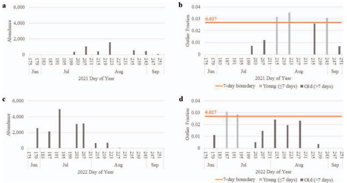
Fig. 11. Wild-caught Coquillettidia perturbans without mites, 2021 trap sites A and B, and 2022 trap site D; abundance (collection size) versus outlier fraction. Collection and scanning details are provided in Table 3; trap site locations are mapped in Fig. 3. The above graphs show: (a) trap sites A and B, 2021 abundance; (b) trap sites A and B, 2021 classification into young or old cohorts based on the calculated 7-day boundary outlier fraction (0.027) from Fig. 9; (c) trap site D, 2022 abundance; and (d) trap site D, 2022 classification into young or old cohorts based on the calculated 7-day boundary outlier fraction (0.027) from Fig. 9.
