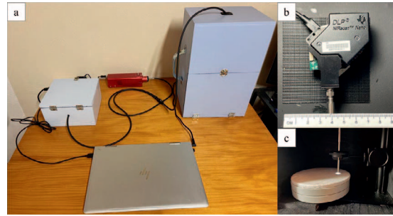
Fig. 2. Spectroscopy setup. (a) Full setup showing cabinetry and fixed light source. (b) Spectrometer with chassis and probe leg attached. (c) Microscope stand with probe and reflectance standard disk.
