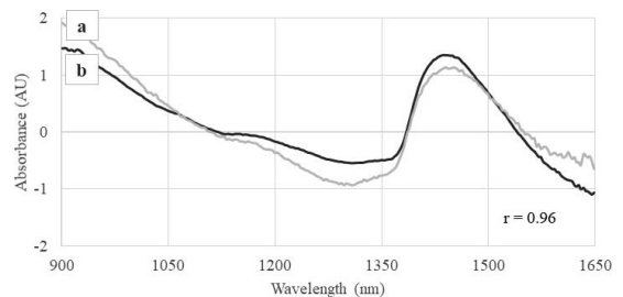
Fig. 9. Spectral averages illustrating the strong correlation between laboratory-reared and wild-caught mosquitoes. (a) This study, Tufts laboratory-reared day-old Aedes aegypti ( n = 6 ). (b) Wild-caught Coquillettidia perturbans , trap site A, collected with a miniature Centers for Disease Control and Prevention (CDC) light trap with CO 2 as an attractant, July 20, 2021 ( n = 120 ).
