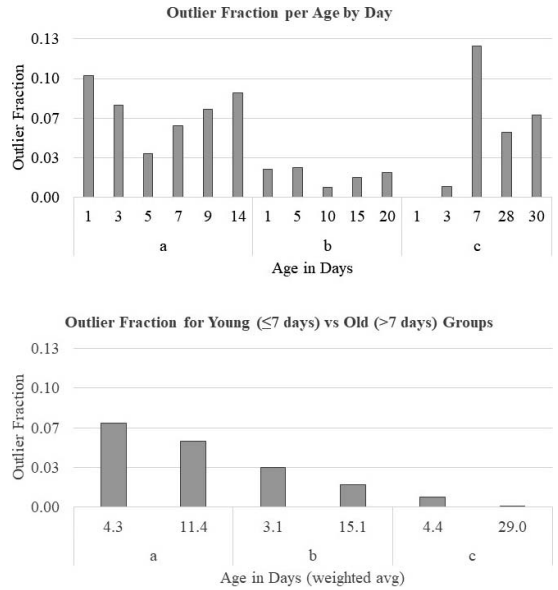
Fig. 5. Outlier fraction for female laboratory-reared mosquitoes by age in days and weighted average age in days. (a) Sikulu et al. (2014): Anopheles gambiae s.l., n = 295 . (b) Sikulu-Lord et al. (2016): Aedes aegypti , n = 225 . (c) This study: Ae. aegypti , n = 60 .
